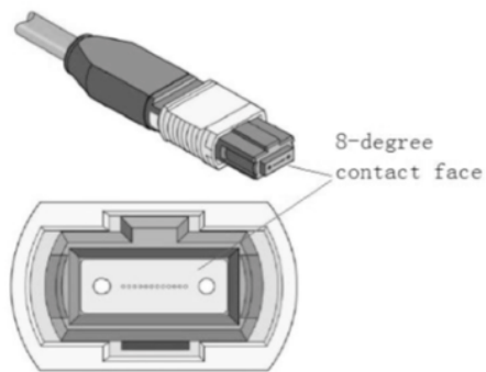
Figure 22 MTP/APC Cable
